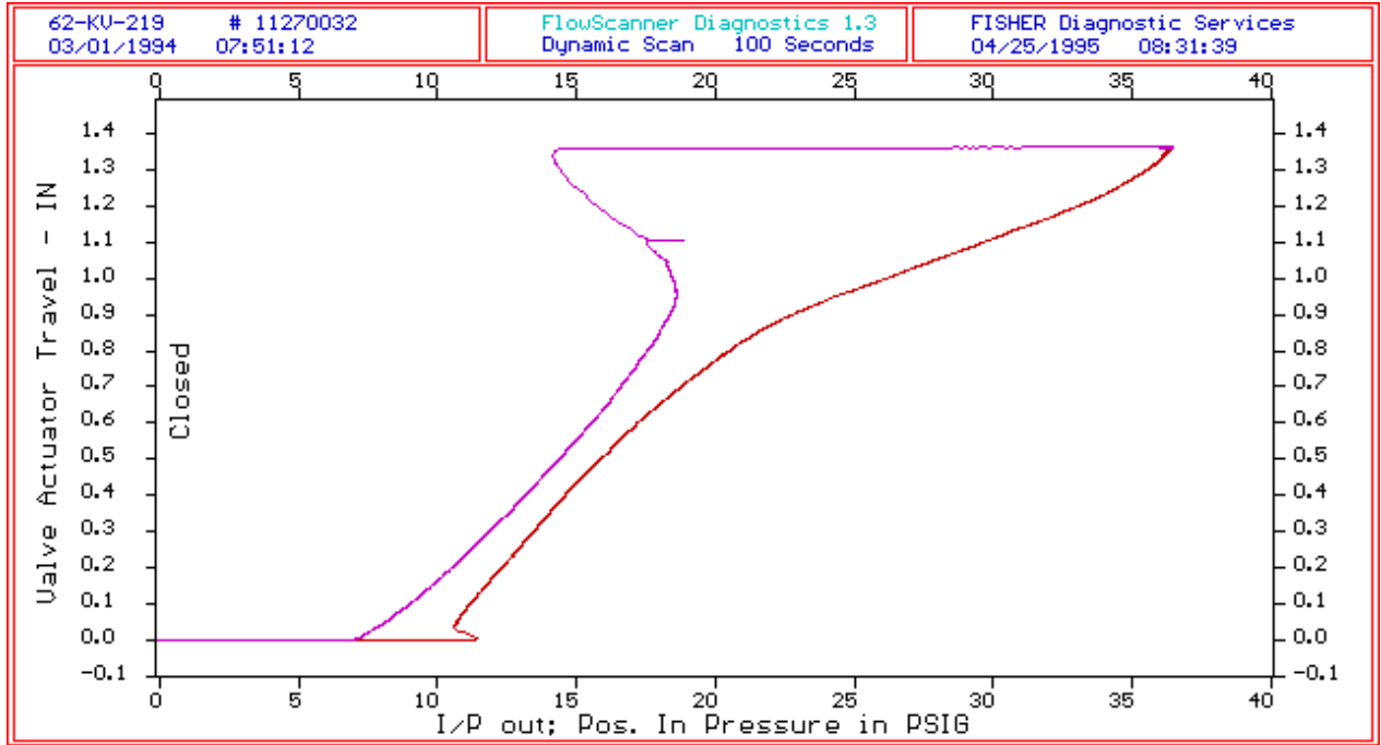
Figure C-10 Positioner Bellows
