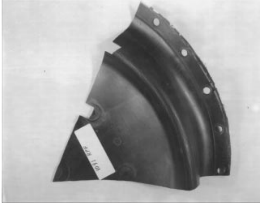
Figure 7-25 Photograph of Crazed Surface of a Section of an OV Diaphragm Removed from Service during ISI
