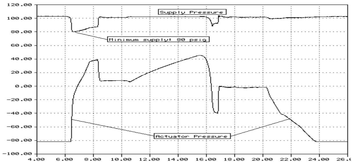
Figure C-2 After—Larger Supply Tubing
