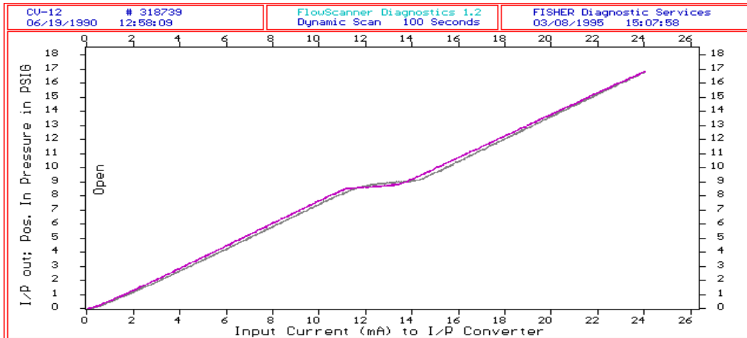
Figure C-8 I/P Calibration
