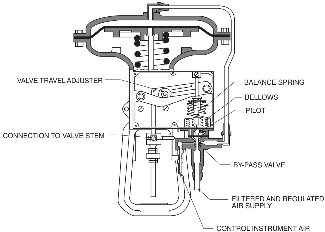
Figure 2-15 Pneumatic Positioner
