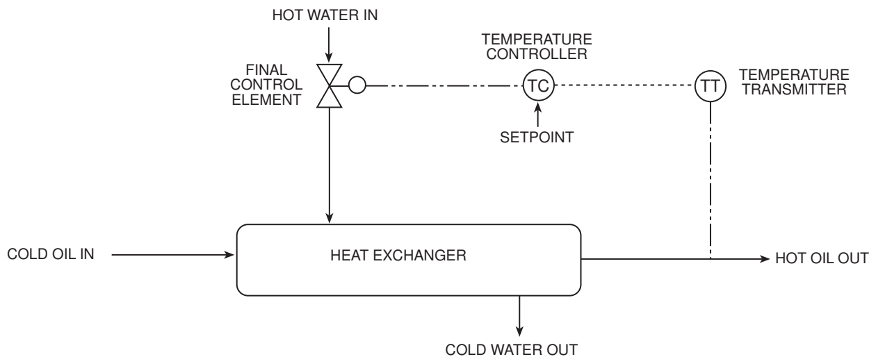
Figure 2-9 Closed Loop Elements
