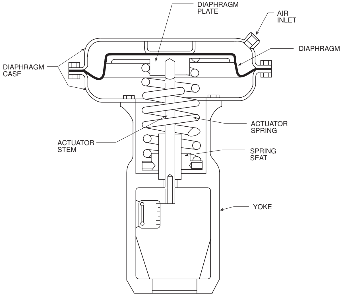
Figure 2-1 Direct-Acting Actuator
