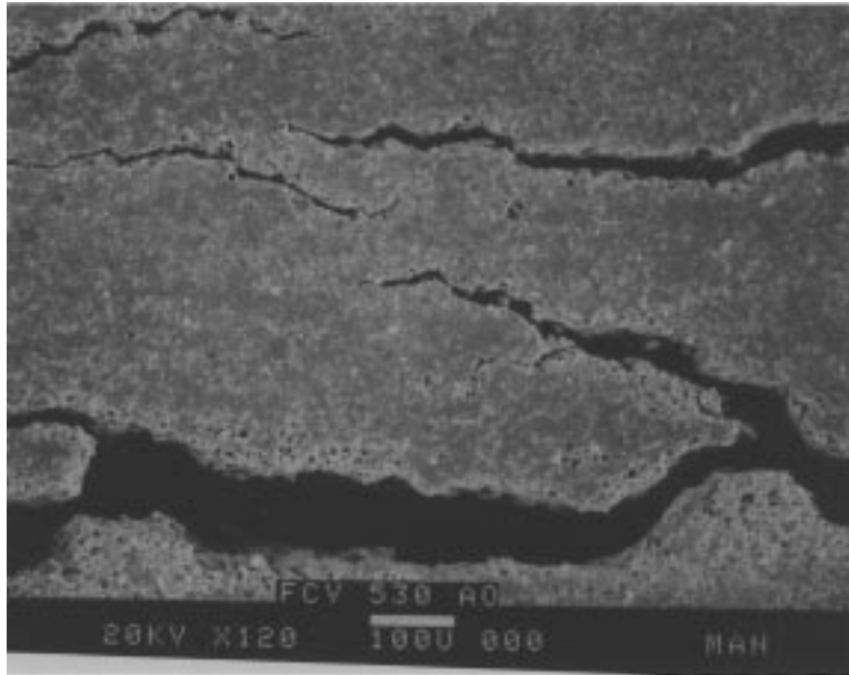
Figure 7-13 Solvent-Attacked Diaphragm, Showing the Porosity Resulting from Dissolution of the Rubber
