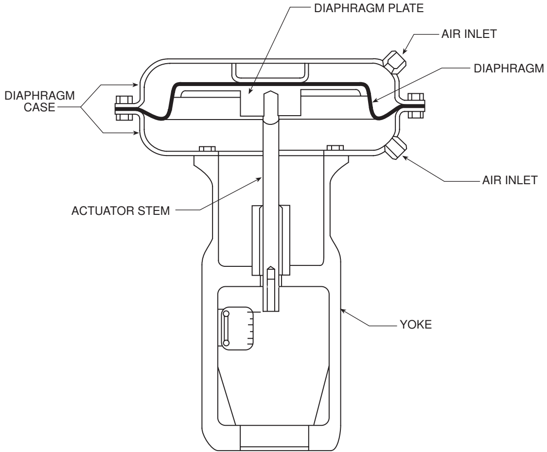
Figure 2-3 Springless-Type Actuator
